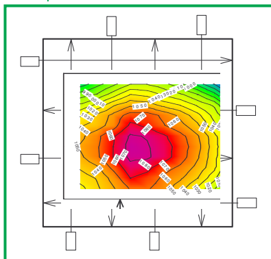
Flame Temperature Distribution 2D (FTD-2D)
