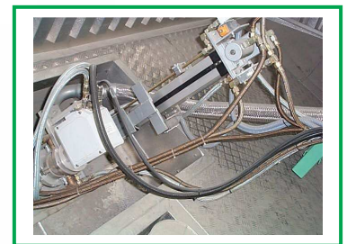
PYROINC256-IR-camera system for control the drying and combustion grate zone
