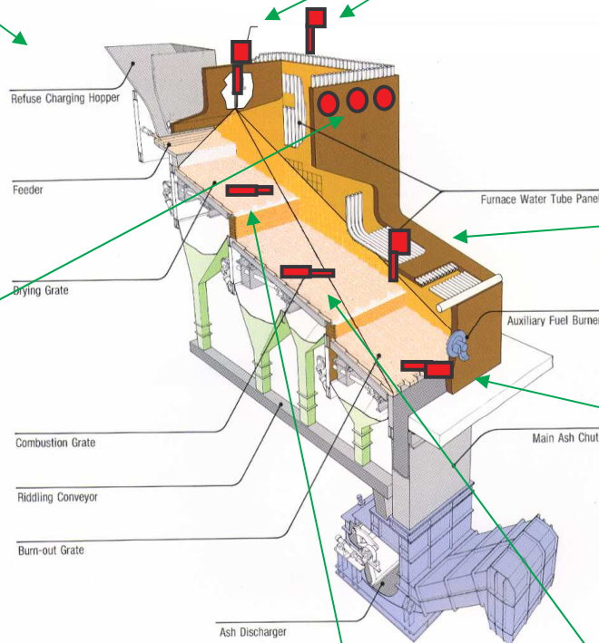
WBFDs-Waste-Bunker-Fire-Detection-System
